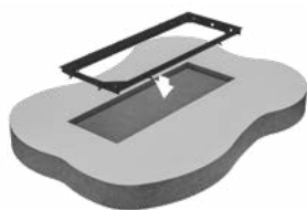
Cornice ad incasso cm 249x90xH18 In ground frame cm 249x90xH18
